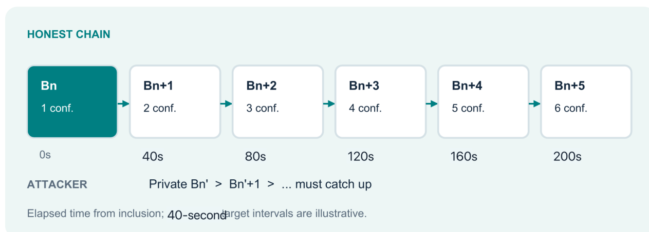
Figure 3B. Security accumulation across 40-second confirmations
