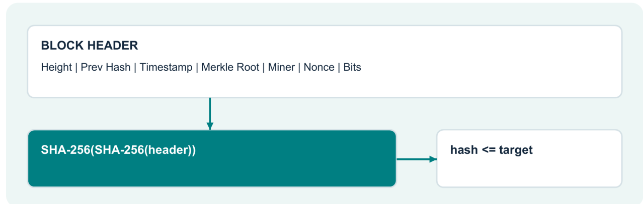
Figure 3. Proof-of-work over the block header
