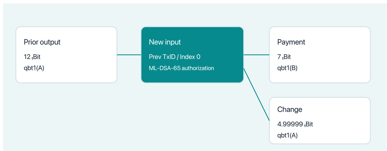
Figure 1. Transfer of ownership through chained outputs
